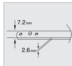
Screw Type
